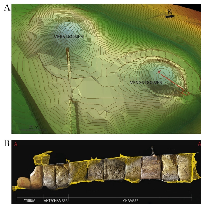
Fig. 3. A. Map of equidistance curves of Viera and Menga mounds. B. Menga Dolmen (cut A, A'): The orthostats of the chamber differ from the rest (antechamber and atrium).
