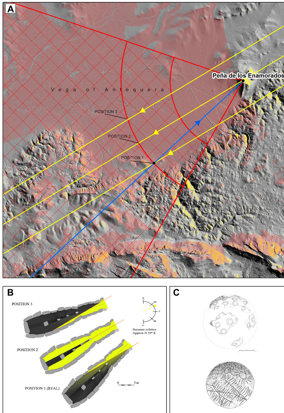
Fig. 11. A. Digital terrain map with the location of the Menga Dolmen (position 1) and its orientation to the Peña de los Enamorados, represented by a blue line. The yellow lines show the direction of the sun at the sunrise on the summer solstice. The yellow hues on the terrain are the sunlit areas at that time. The red hues are the areas from which the Peña de los Enamorados can be seen. The squared web in red, would include all the possible areas where the dolmen could have been placed, orientated to the Peña de los Enamorados. Position 2 (and any other point on this yellow line that is within the red squared web) consist of the place or places where the dolmen would be orientated to both the Peña de los Enamorados and the summer solstice. Position 3 (and any other point on this yellow line that is within the red squared web) consist of the place or places where the dolmen would be orientated to the Peña de los Enamorados, but in this case the only lit part is the left (or perfect) side of the dolmen. This side is dark in the rest of the large gallery dolmens. B. Lighting inside the dolmen in the ideal position (position 2) (orientated to the Peña de los Enamorados and the summer solstice) and in each of the symmetrical positions on both sides of the ideal position. C. Neolithic sherds with carved suns motif, from the Poblado de Campos de Cuevas de Almanzora, Almería (Martín Socas et al., 1982, 1986). (For interpretation of the references to colour in this figure legend, the reader is referred to the web version of this article.)
