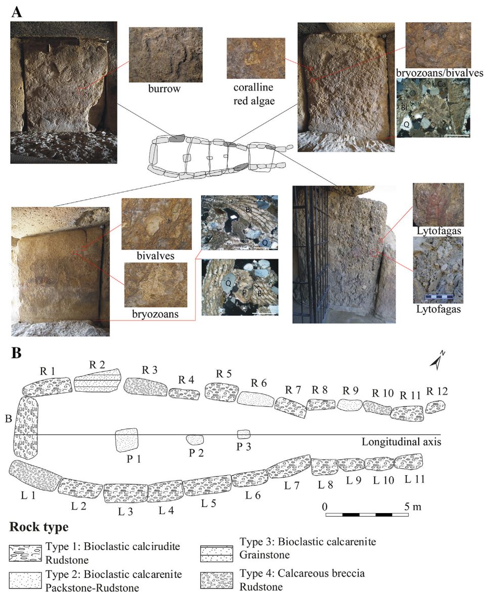
Fig. 5. Menga Dolmen. A. Representation of bioclastic facies (microfacies) of the orthostats. B. Plan of the dolmen with the distribution of the different types of microfacies (L: Left; R: Right; P: Pillar; B: backslap).
