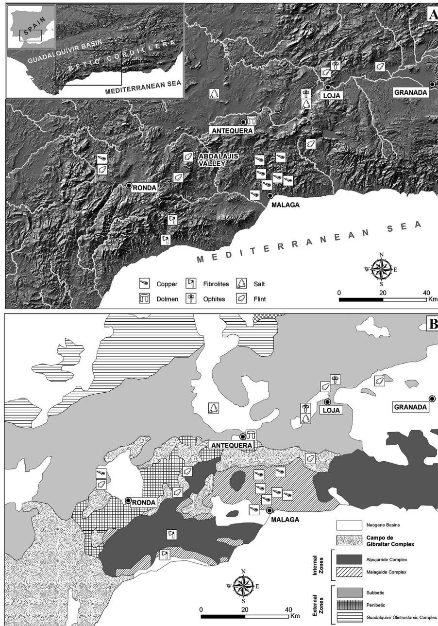
Fig. 1. Location of the Antequera Megalithic Complex, in relation to abiotic resources of its environment.
