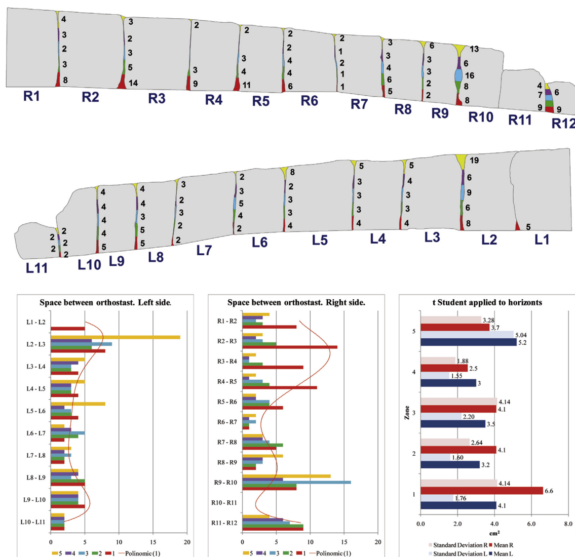
Fig. 8. Spacing between orthostats of the right and left sides.
